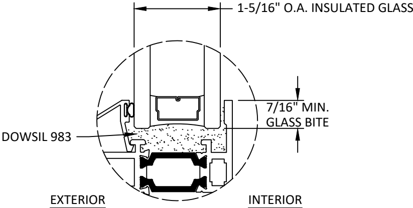
GLAZING DETAIL
