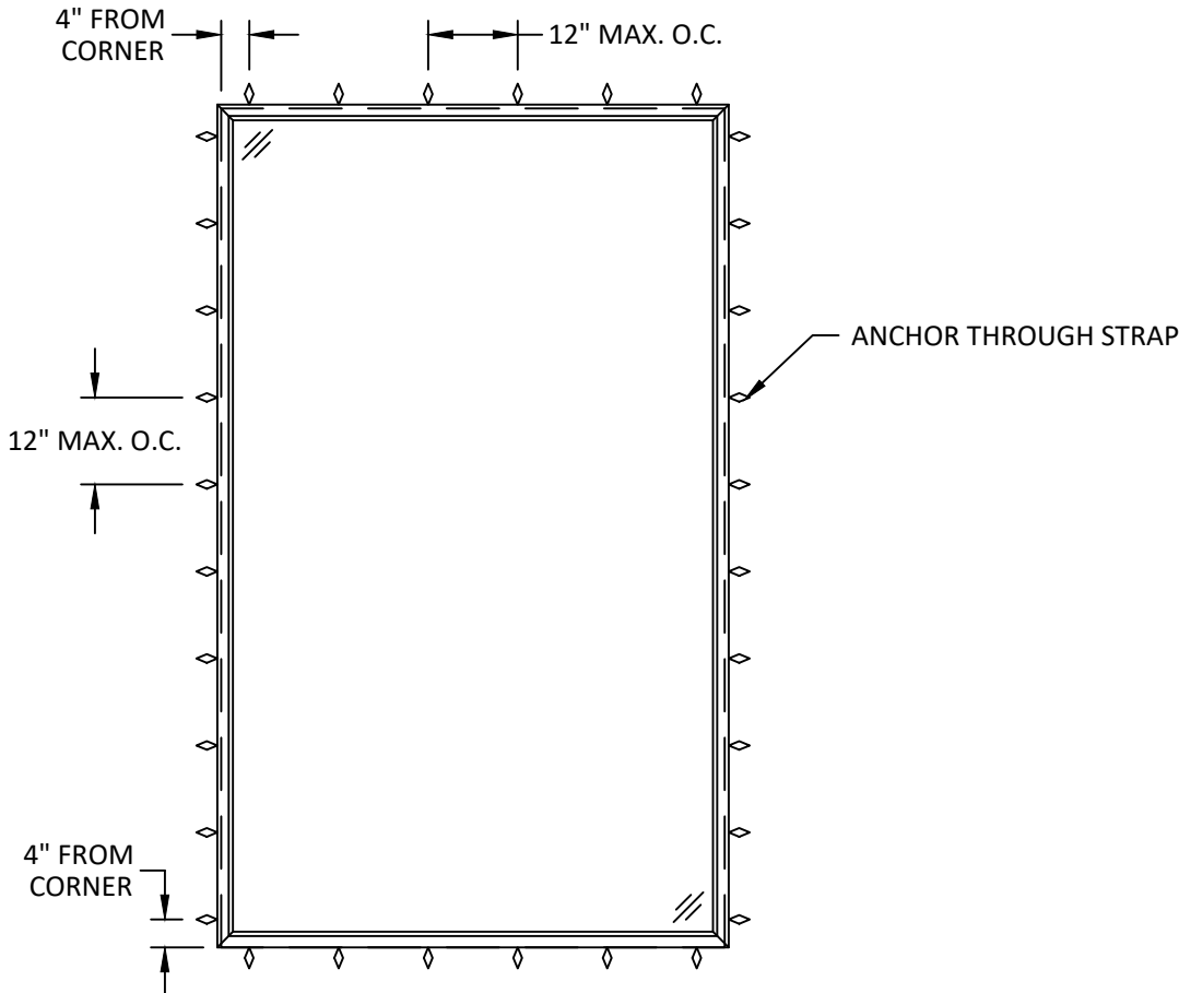
ANCHOR LAYOUT
